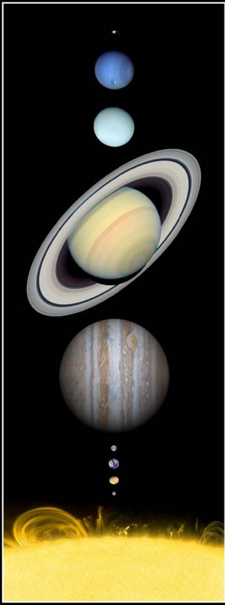
The Sun and Nine Planets
